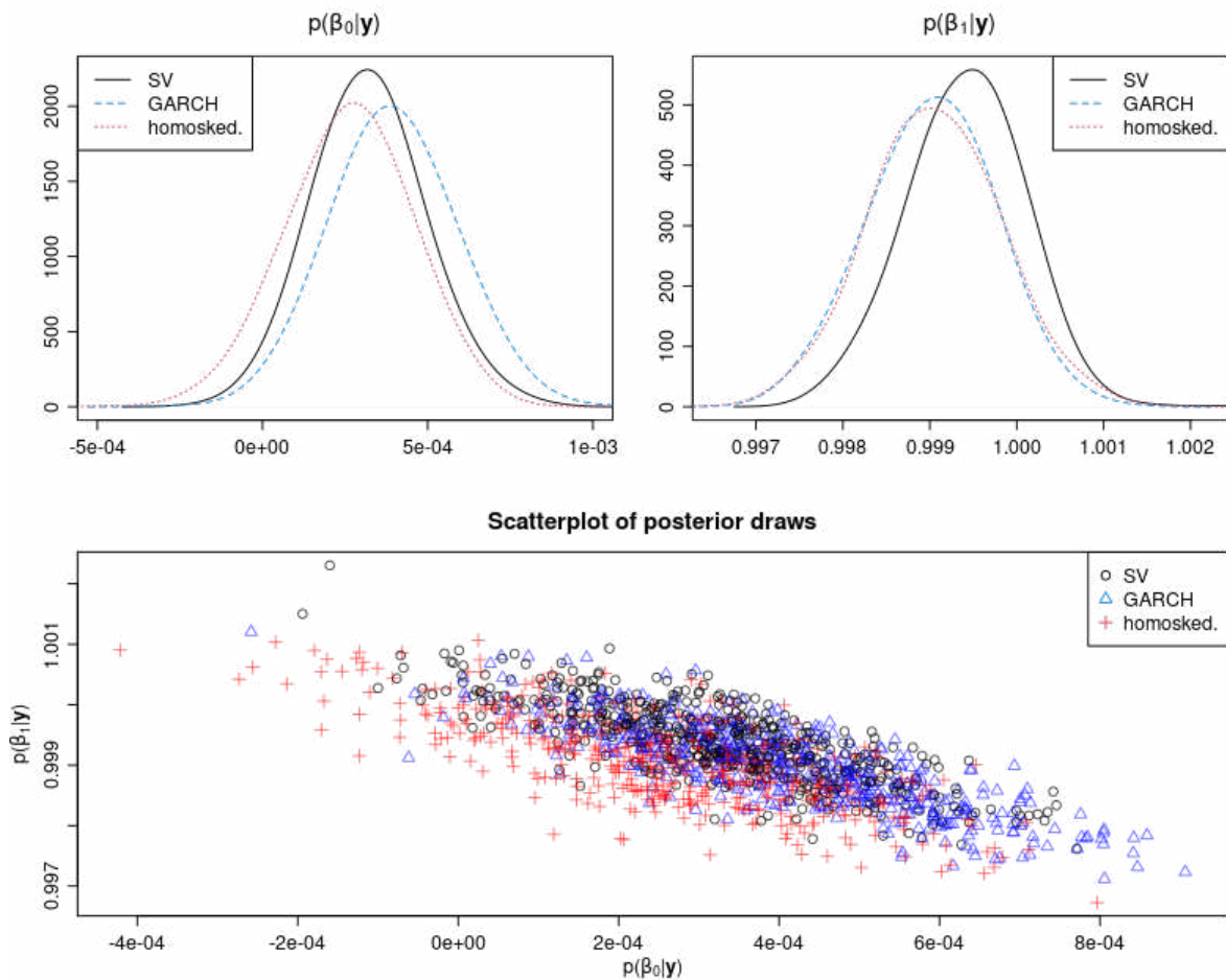
Figure 12: Visualization of the posterior distributions \boldsymbol{\beta}|\mathbf{y} for the model with SV regression residuals, the model with GARCH(1,1) regression residuals, and the model with homoskedastic regression residuals. Top panels: Kernel density estimates of the univariate posterior marginal distributions. Bottom panel: Bivariate scatterplot of posterior draws.
