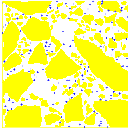
concrete
