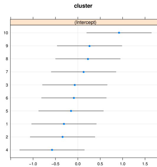
Figure 5: Random effects for the linear mixed-effects model tree in Figure 4.
