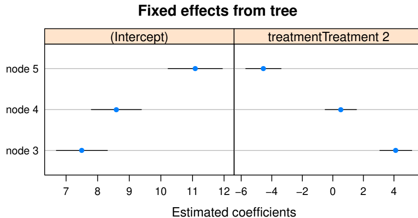
Figure 6: Estimated node-specific fixed effects with error bars.
