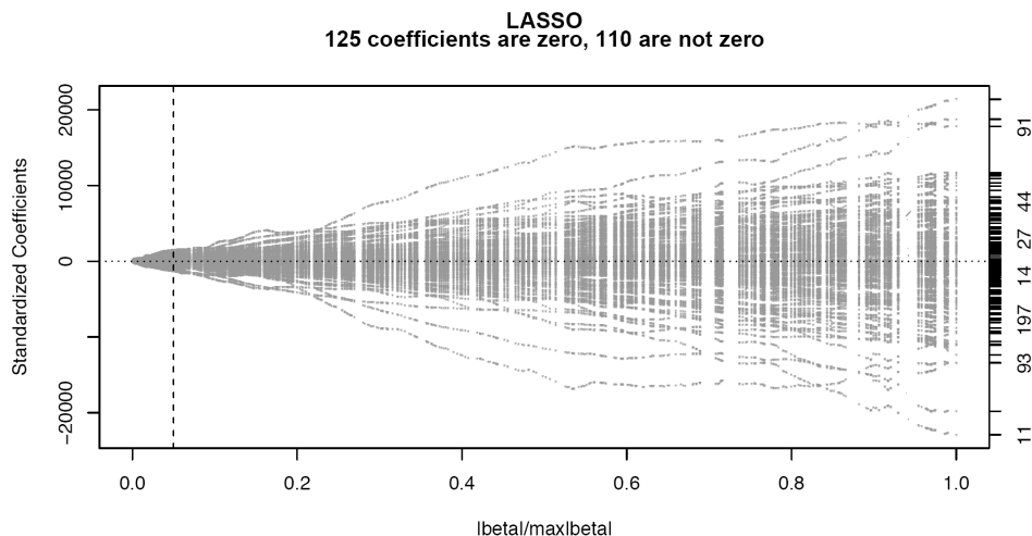
Figure 24: Output of function lassocoef . Development of the Lasso coefficients with increasing fraction. Dashed vertical line: optimal fraction determined before.
