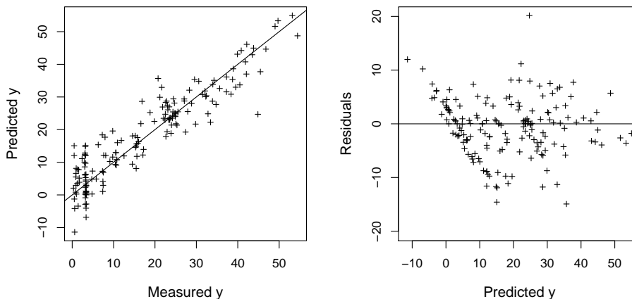
Figure 16: Output of function plotprn . Compare Figures 13 and 14. Left: Predicted versus measured glucose concentrations. Right: Residuals versus predicted values.
