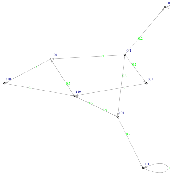
Figure 8: State transition graph of the example probabilistic Boolean network included in BoolNet. Each node represents a state of the network, and each arrow is a possible state transition, annotated by the transition probability.
